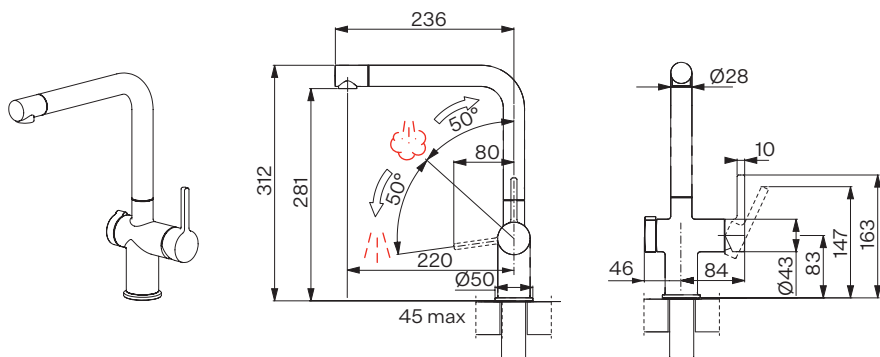
Tap Active Twist L swivel spout
