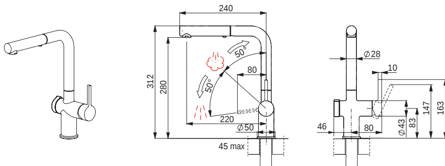
Tap Active Twist pull out 2 jets
