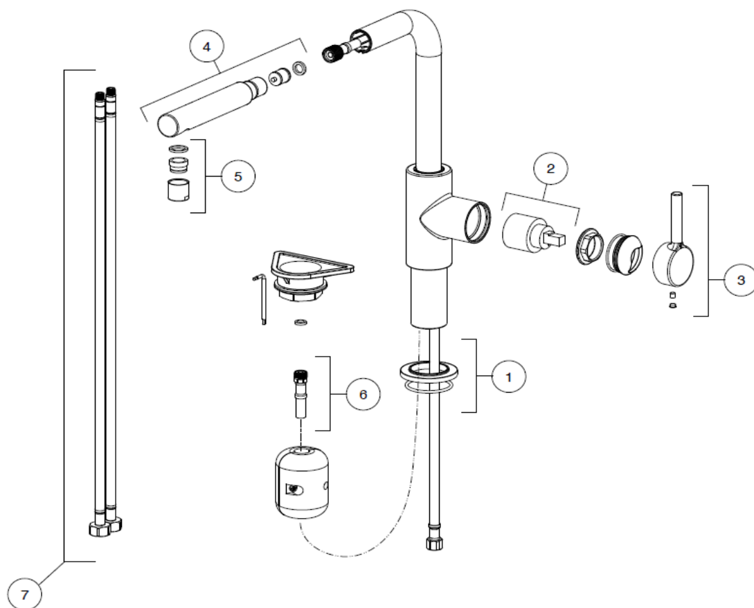
Tap Lina L Pull Out Nozzle HP ST 115.0728.486
