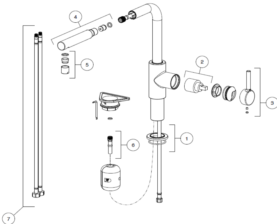
Tap Lina L Pull Out Nozzle HP CO 115.0728.488
