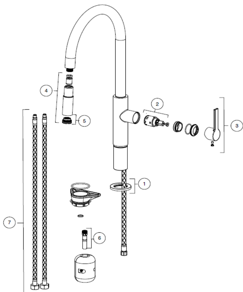
Tap Maris Slim J Pull Down HP MB 115.0728.389
