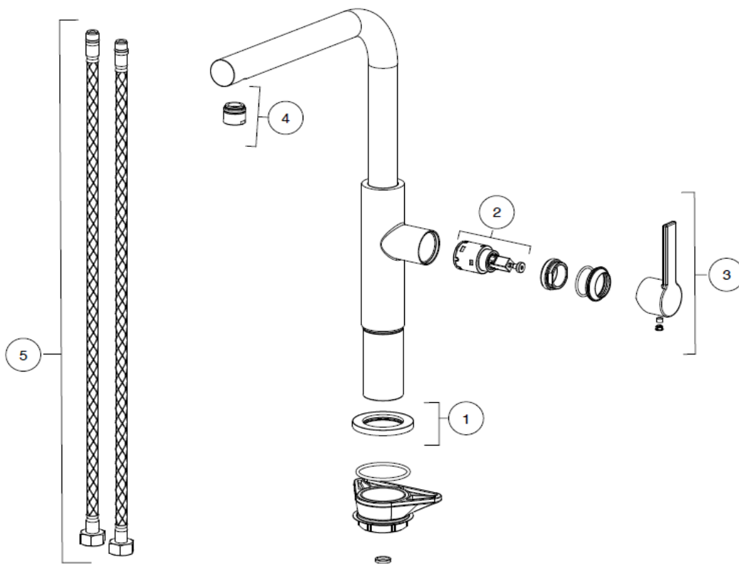
Tap Maris Slim L Swivel side HP MB 115.0728.391
