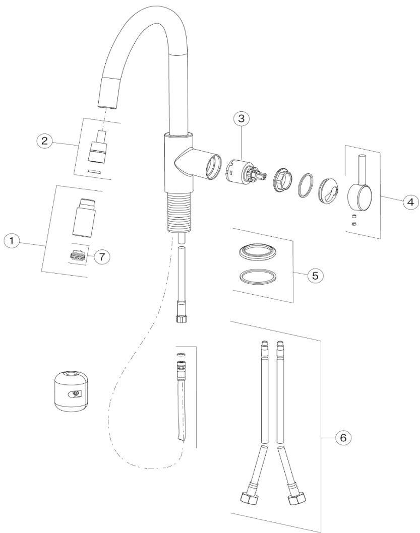
Lina Pull Down nozzle side HP Stonegrey (EU version)
