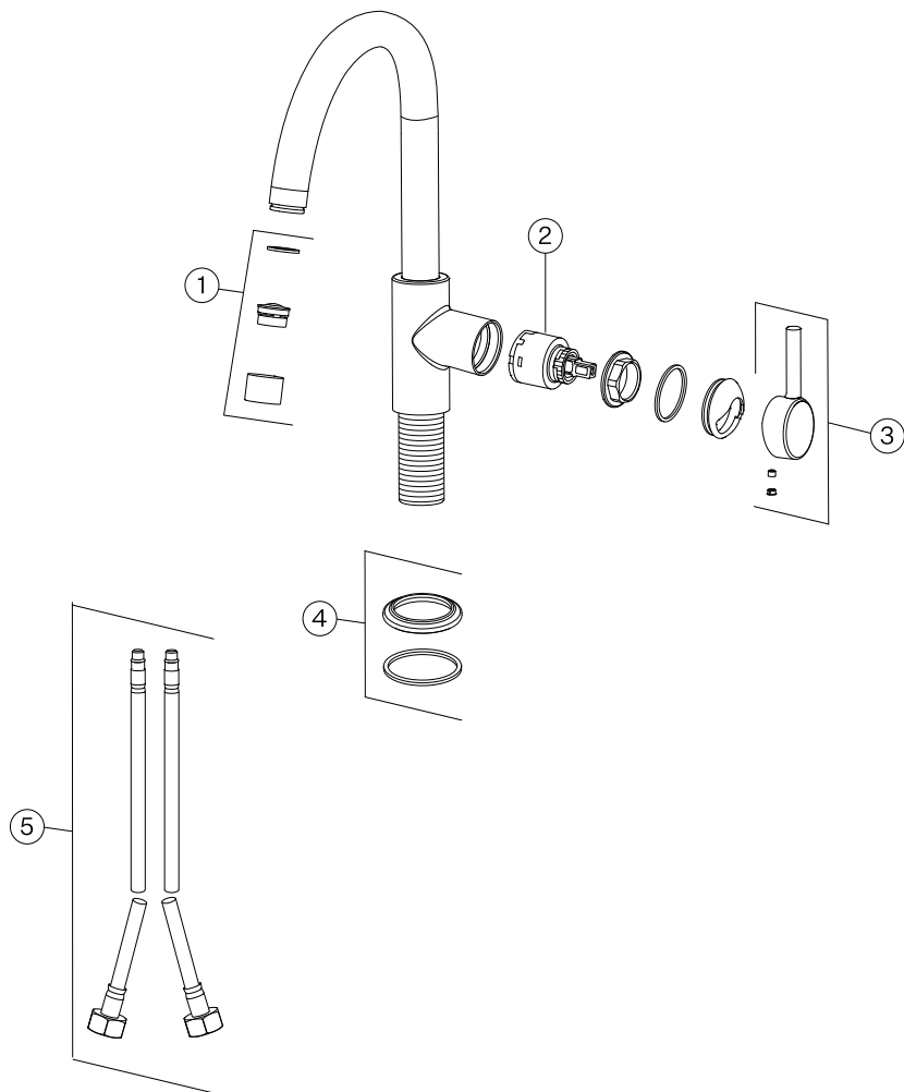
Lina Swivel XL Side HP Polar White (EU version)
