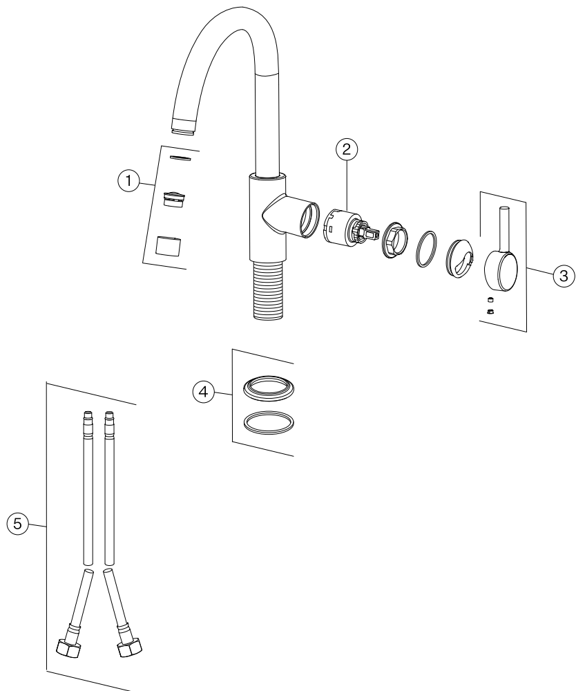
Lina Swivel XL Side HP Matte Black (EU version)
