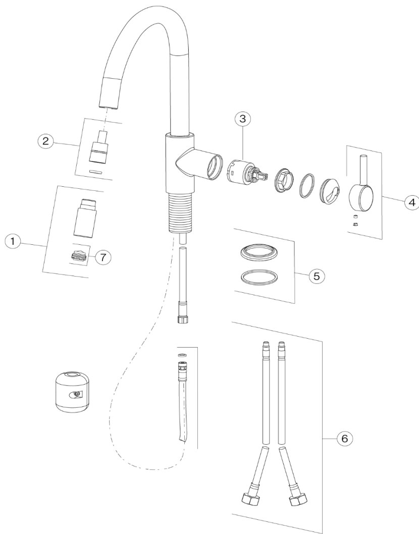
Lina Pull Down nozzle side HP Coffee (EU version)
